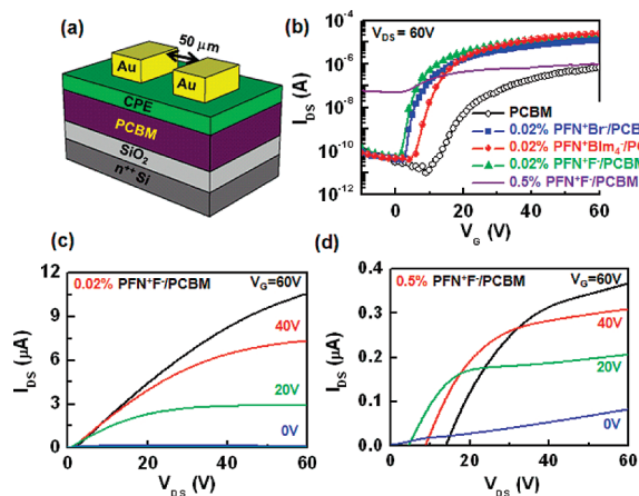
Figure 1. (a) OTFT test device. (b) Transfer characteristics at V_{DS} = 60 V as a function of counterion and concentration (for only \text{PFN}^+\text{F}^- ). (c, d) Output characteristics with \text{PFN}^+\text{F}^- layers deposited from 0.02% and 0.5% methanol solutions, respectively.
